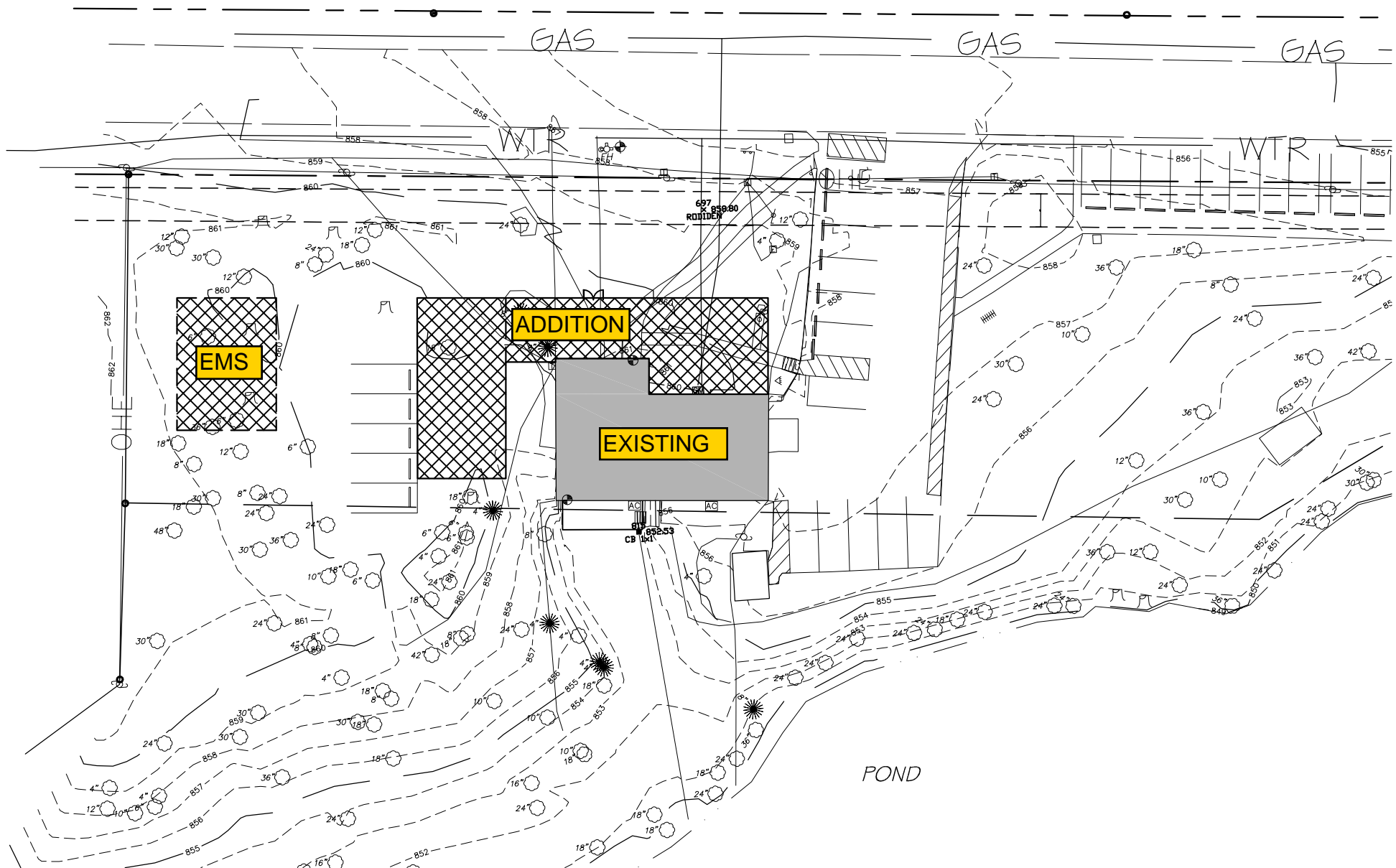
1 SITE PLAN - PHASED OPTION 1/16" = 1'-0"
