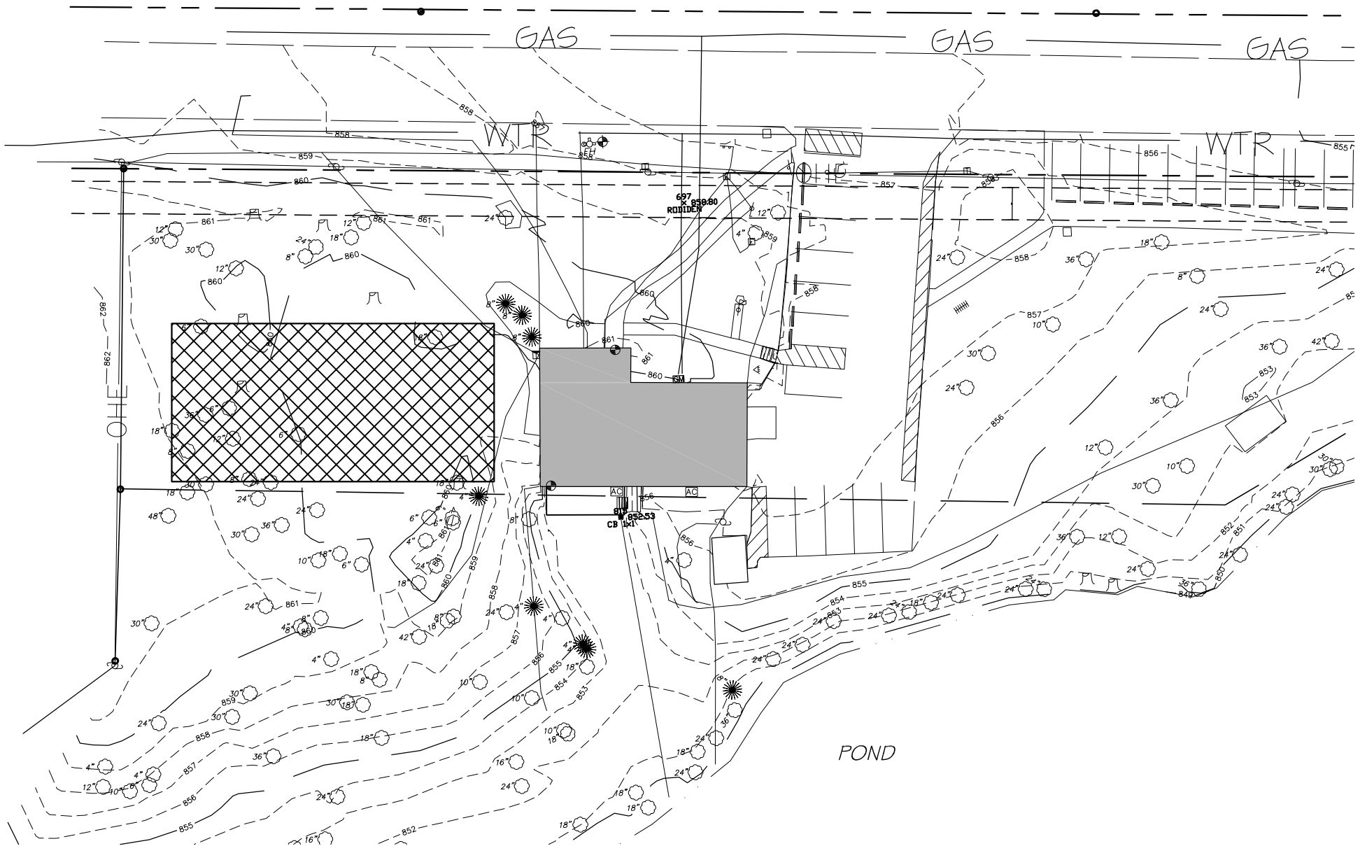
1 SITE PLAN - SEPARATE BUILDING 1/16" = 1'-0"
