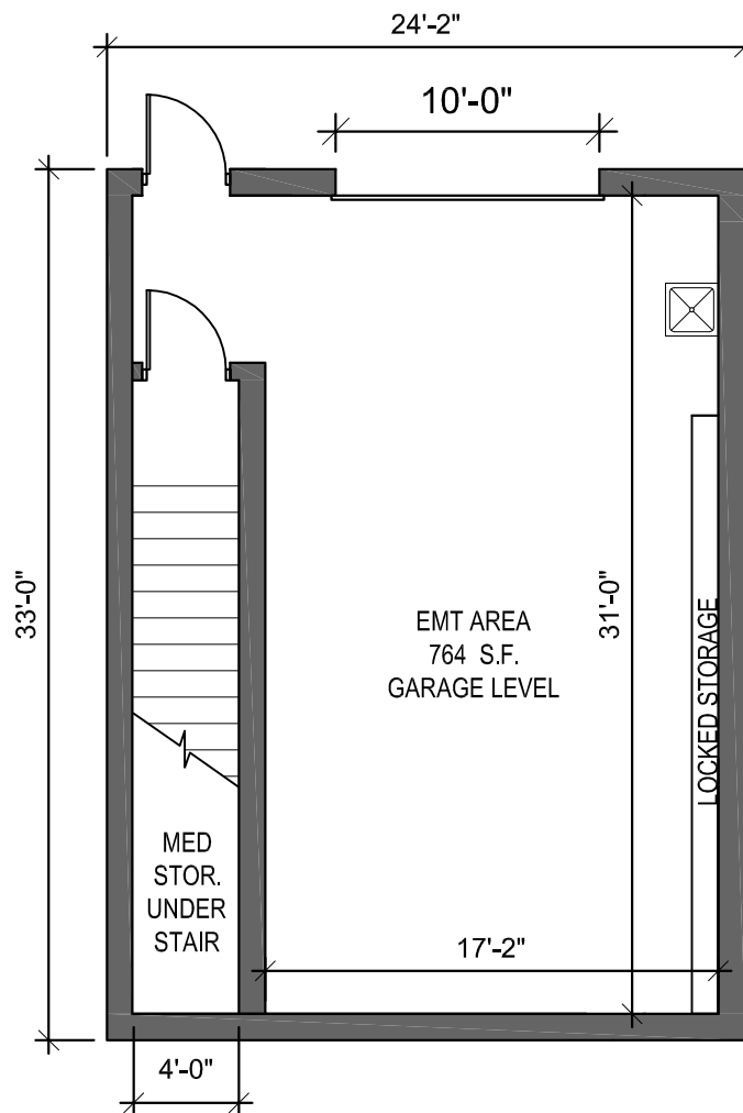
2 PROPOSED GARAGE FLOOR PLAN - EMS 1/8" = 1'-0"
